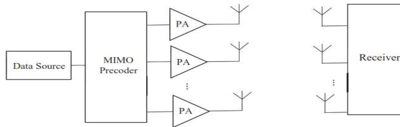
Figure 1. Multiple Input Multiple Output (MIMO) Structure
