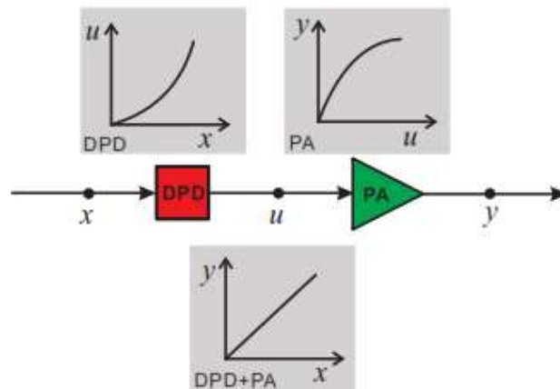
Figure 9. Principles of Pre-distortion Method (Guan & Zhu, 2017).
