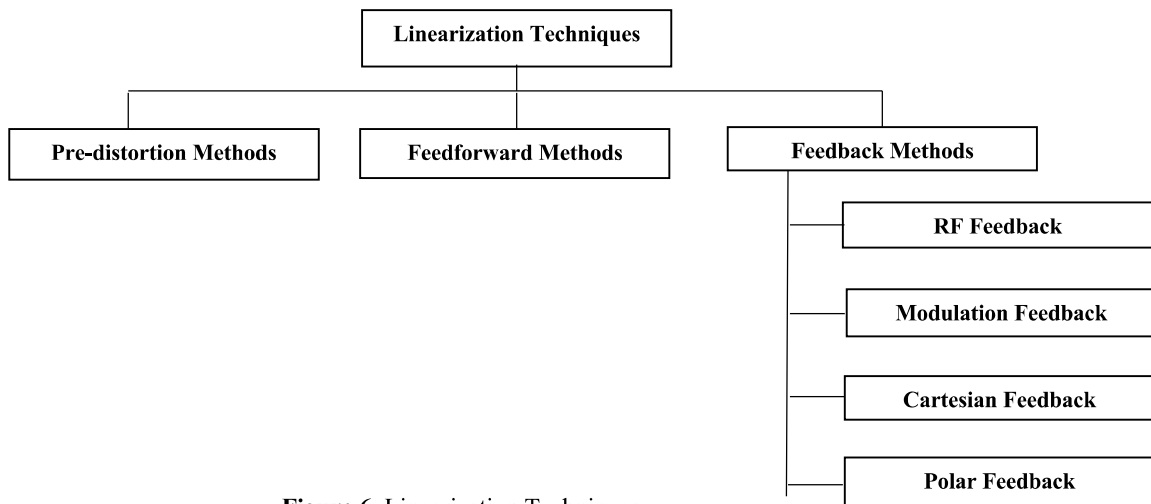
Figure 6. Linearization Techniques
