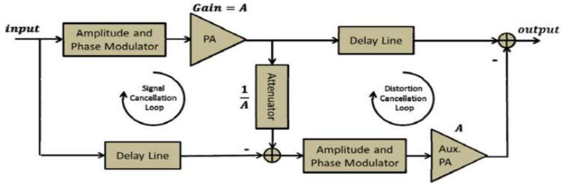
Figure 7. Block Diagram of Feedforward Linearization Technique (Cheaito, 2017).
