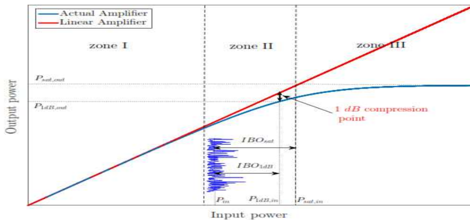
Figure 5. Power Amplifier Characteristics: Linear, Compression and Saturation Zones.
