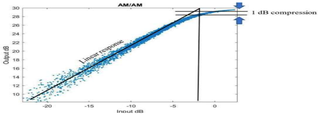
Figure 4. Power Amplifier Output Response.
