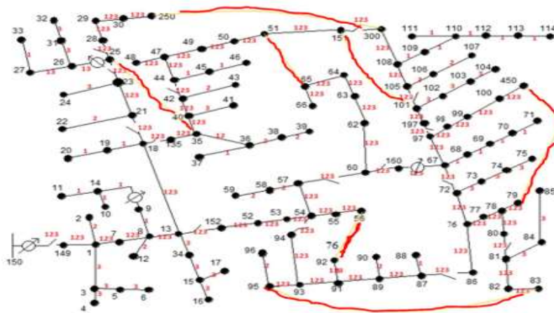
Figure 2: Optimally reconfigured IEEE 123-bus radial distribution system.
